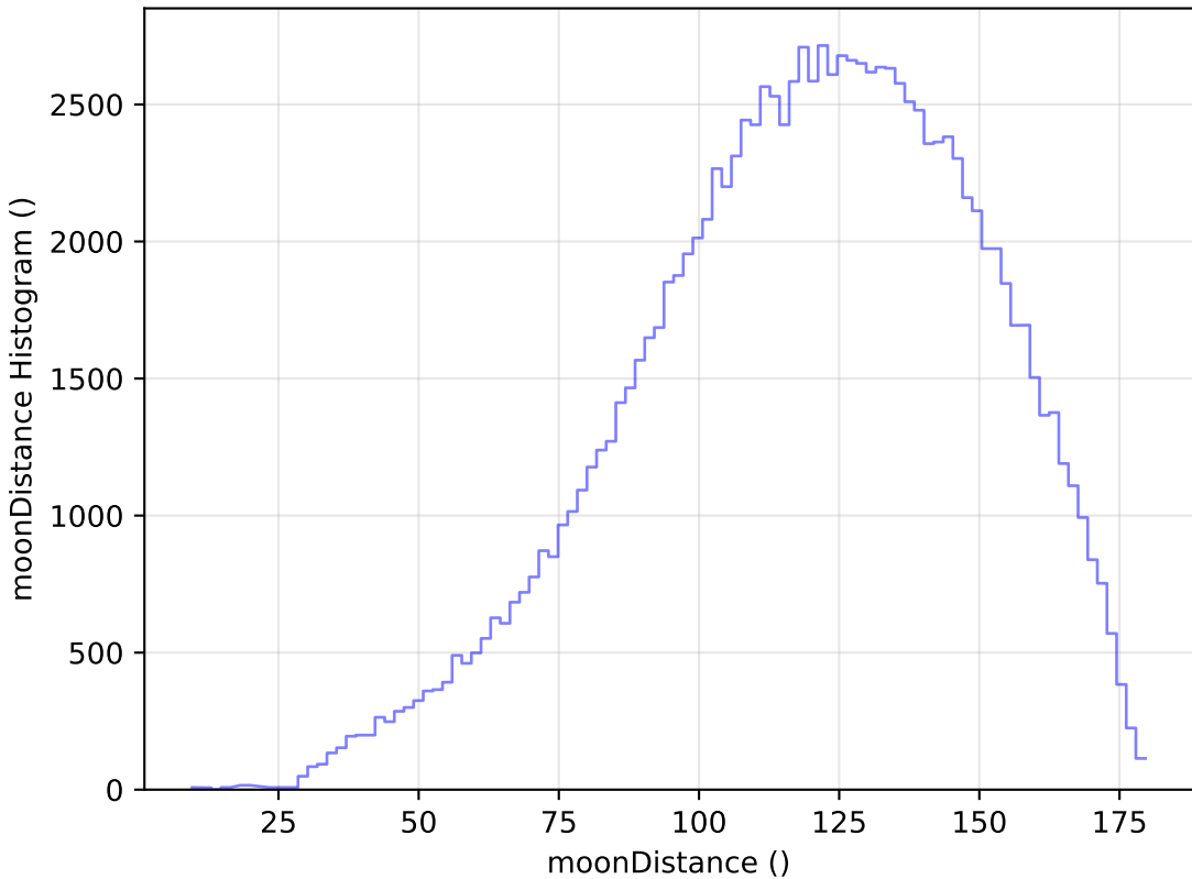
too_elab_r8_d3_giz_v3.4_10yrs WFD u band: moonDistance Histogram
