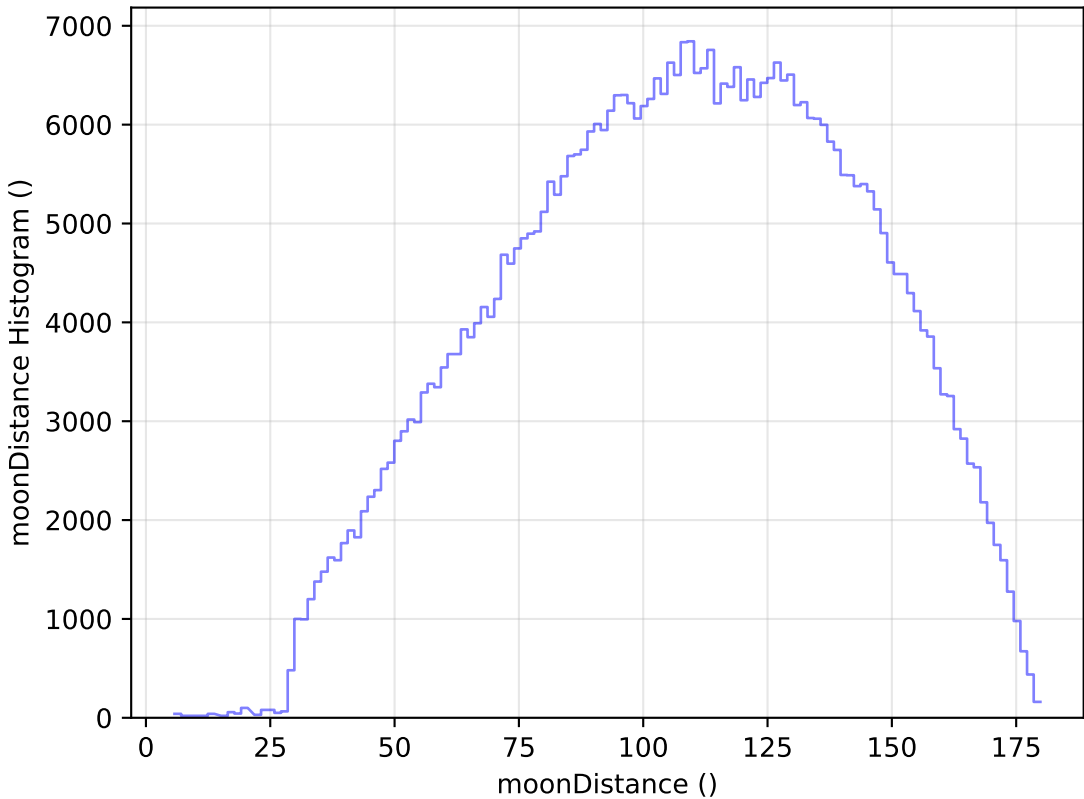
too_elab_r8_d3_giz_v3.4_10yrs WFD r band: moonDistance Histogram
