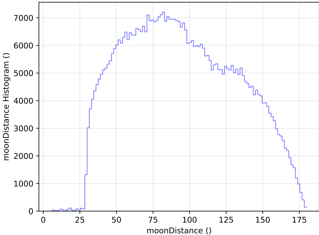
too_elab_r8_d3_giz_v3.4_10yrs WFD i band: moonDistance Histogram
