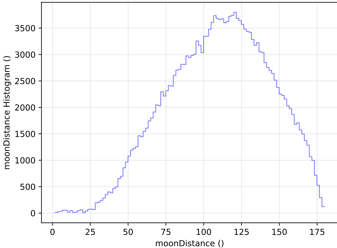
too_elab_r8_d3_giz_v3.4_10yrs WFD g band: moonDistance Histogram
