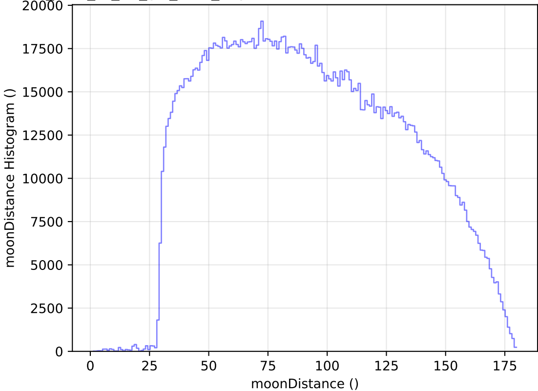
too_elab_r8_d3_giz_v3.4_10yrs WFD all bands: moonDistance Histogram
