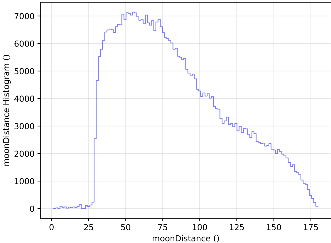
too_elab_r8_d3_giz_v3.4_10yrs All sky z band: moonDistance Histogram
