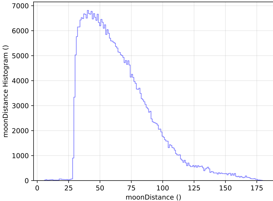
too_elab_r8_d3_giz_v3.4_10yrs All sky y band: moonDistance Histogram
