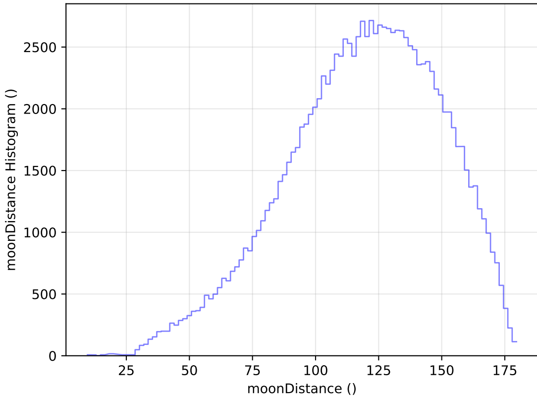
too_elab_r8_d3_giz_v3.4_10yrs All sky u band: moonDistance Histogram
