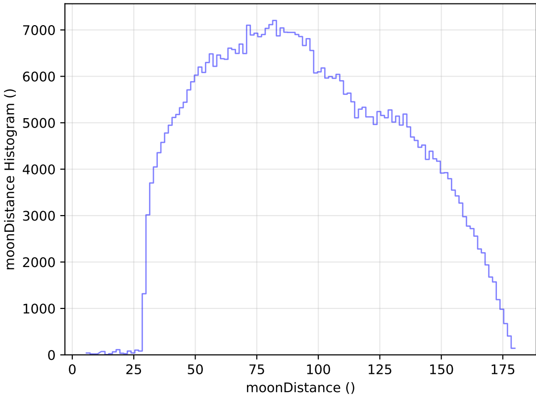
too_elab_r8_d3_giz_v3.4_10yrs All sky i band: moonDistance Histogram
