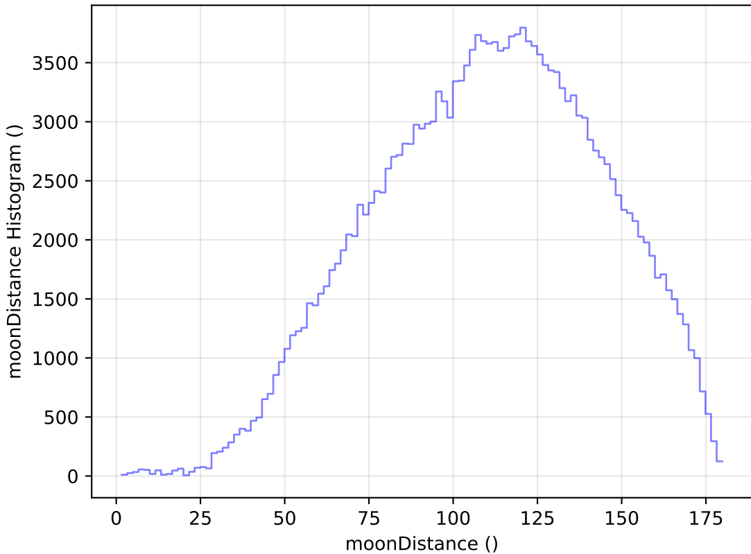
too_elab_r8_d3_giz_v3.4_10yrs All sky g band: moonDistance Histogram
