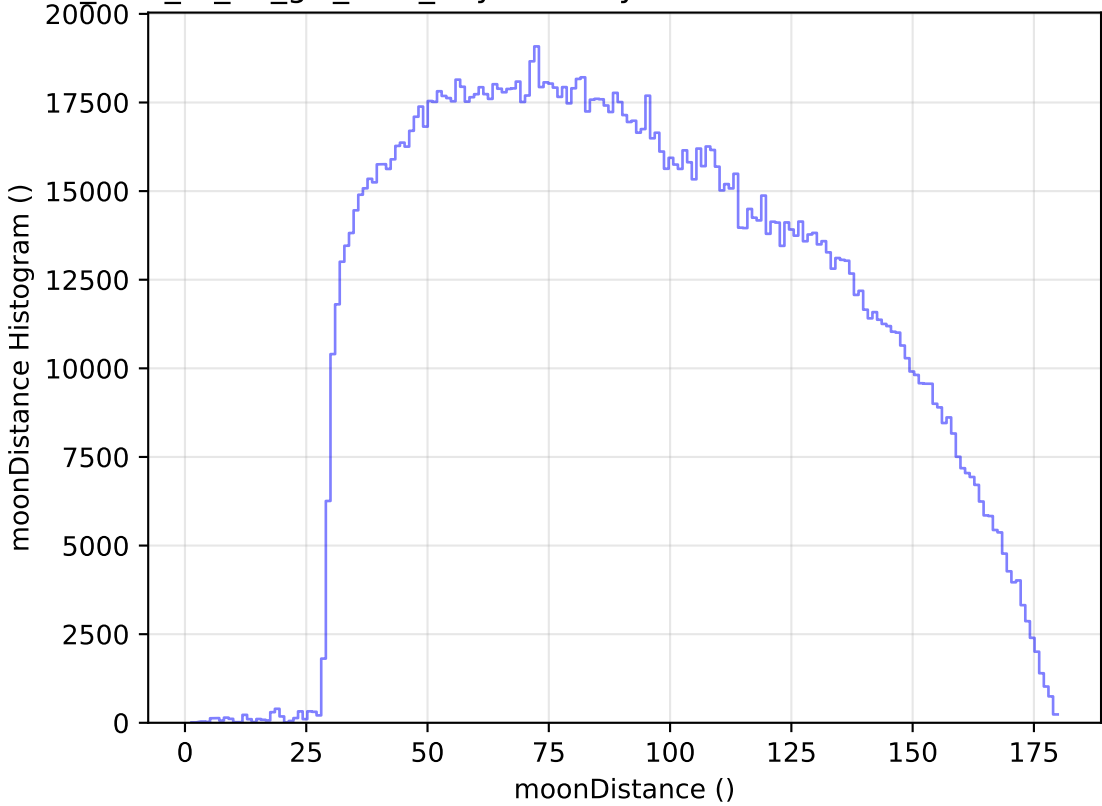
too_elab_r8_d3_giz_v3.4_10yrs All sky all bands: moonDistance Histogram
