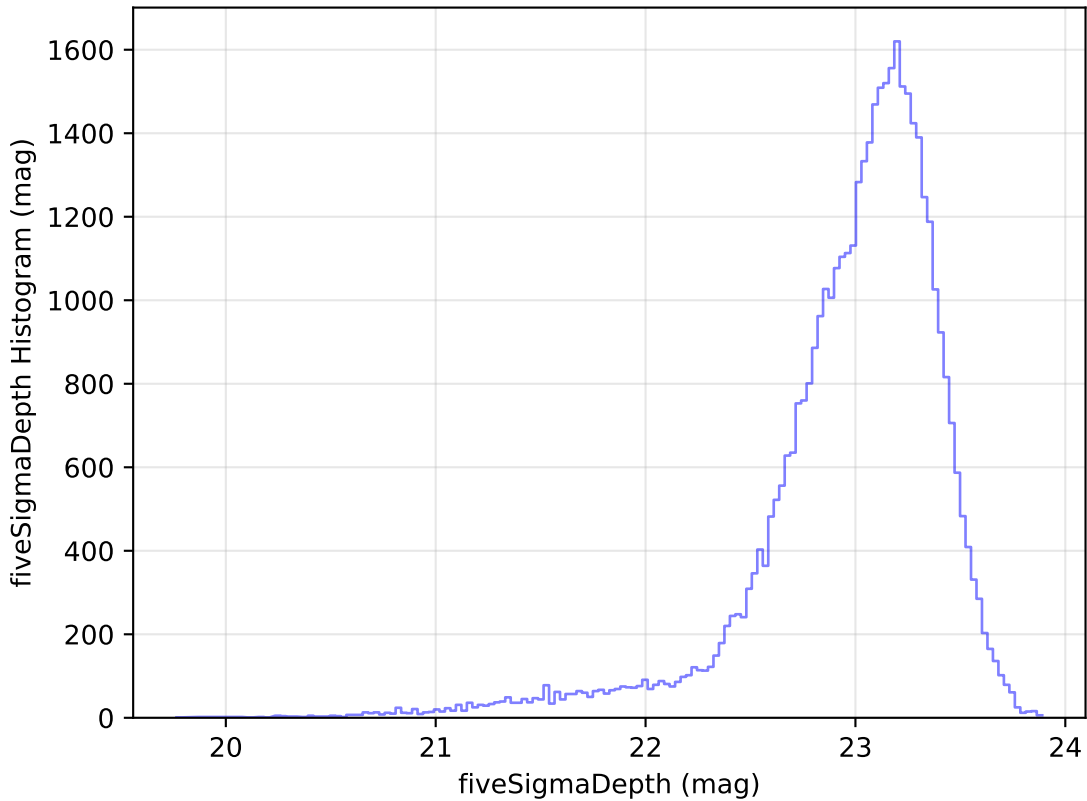
too_elab_r8_d3_giz_v3.4_10yrs Yr 1 z band: fiveSigmaDepth Histogram
