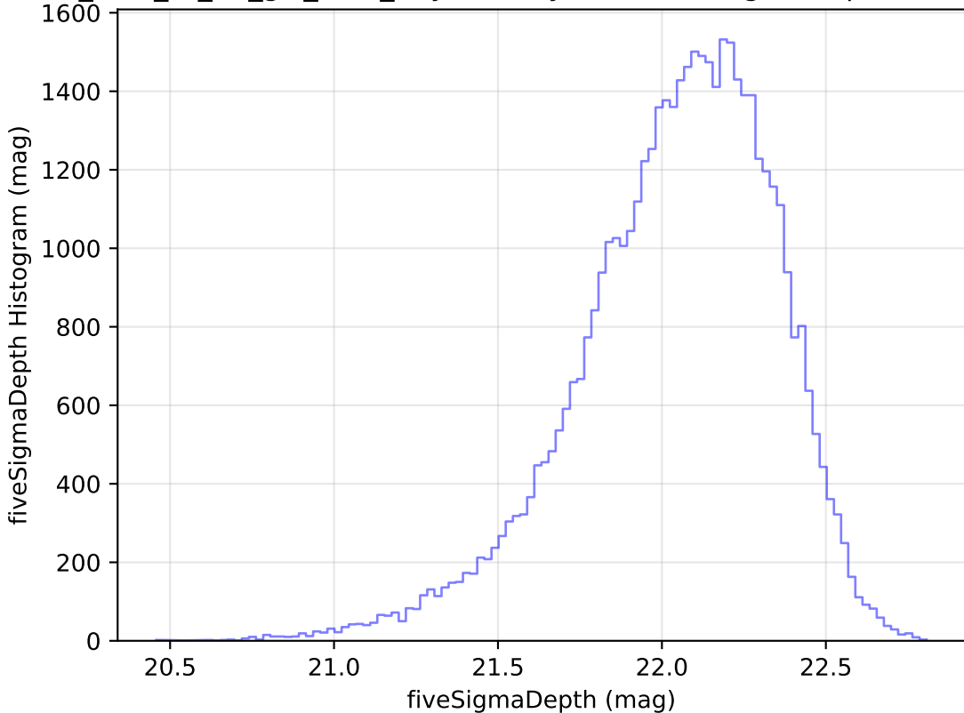
too_elab_r8_d3_giz_v3.4_10yrs Yr 1 y band: fiveSigmaDepth Histogram
