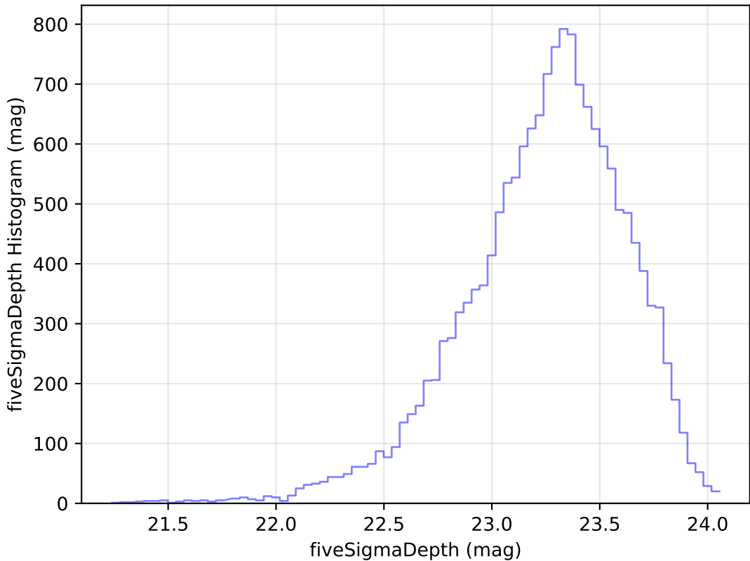
too_elab_r8_d3_giz_v3.4_10yrs Yr 1 u band: fiveSigmaDepth Histogram
