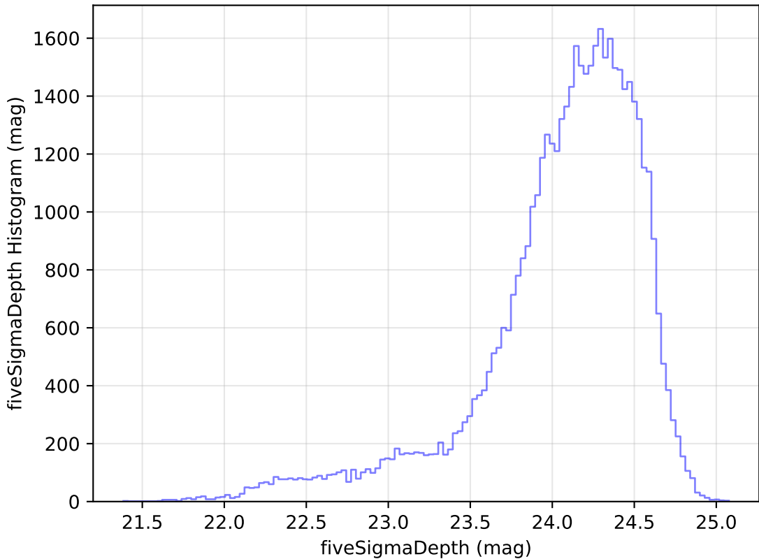
too_elab_r8_d3_giz_v3.4_10yrs Yr 1 r band: fiveSigmaDepth Histogram
