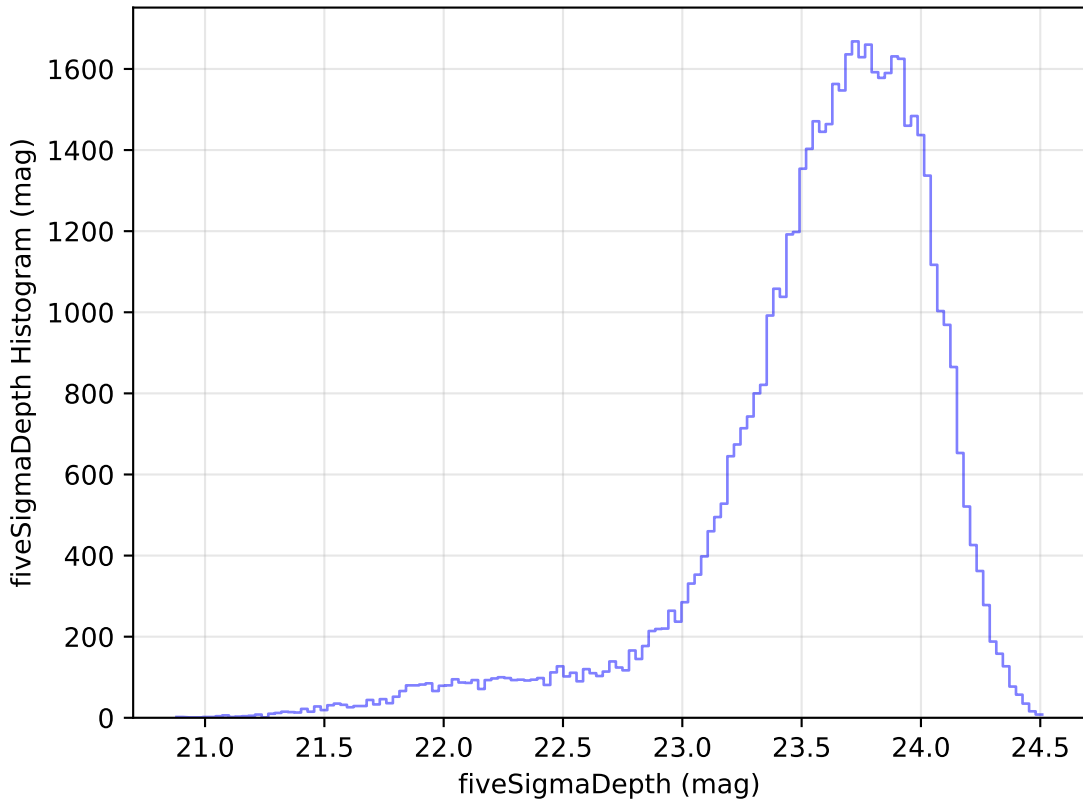
too_elab_r8_d3_giz_v3.4_10yrs Yr 1 i band: fiveSigmaDepth Histogram
