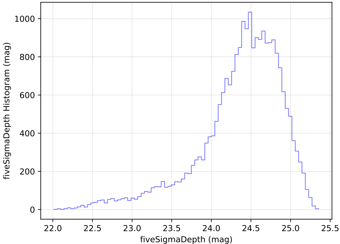
too_elab_r8_d3_giz_v3.4_10yrs Yr 1 g band: fiveSigmaDepth Histogram
