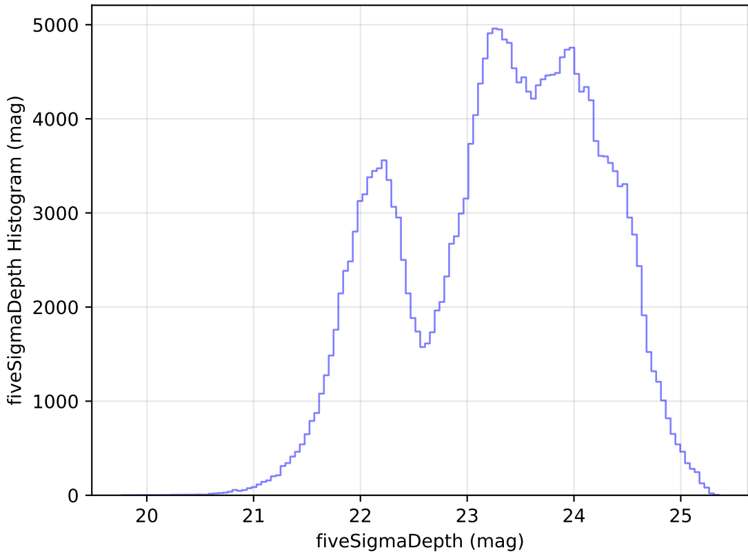
too_elab_r8_d3_giz_v3.4_10yrs Yr 1 all bands: fiveSigmaDepth Histogram
