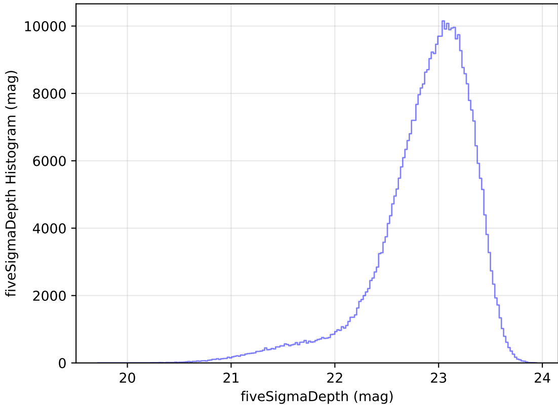
too_elab_r8_d3_giz_v3.4_10yrs WFD z band: fiveSigmaDepth Histogram
