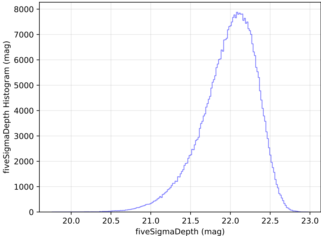
too_elab_r8_d3_giz_v3.4_10yrs WFD y band: fiveSigmaDepth Histogram
