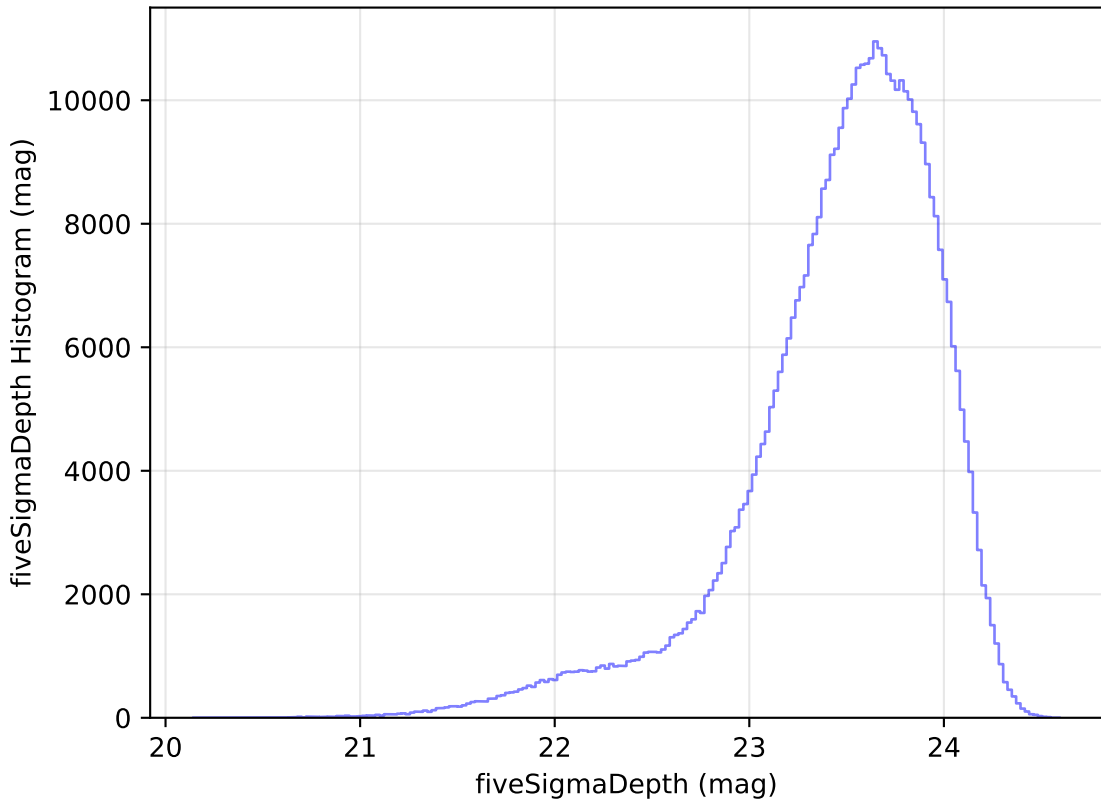
too_elab_r8_d3_giz_v3.4_10yrs WFD i band: fiveSigmaDepth Histogram
