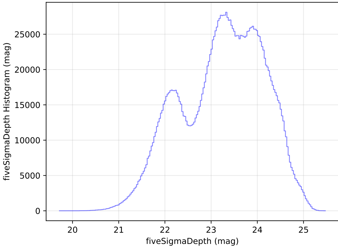
too_elab_r8_d3_giz_v3.4_10yrs WFD all bands: fiveSigmaDepth Histogram
