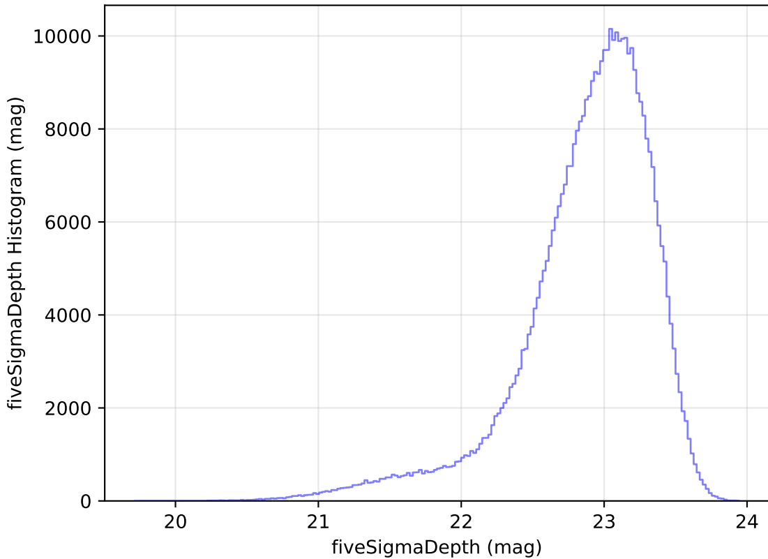
too_elab_r8_d3_giz_v3.4_10yrs All sky z band: fiveSigmaDepth Histogram
