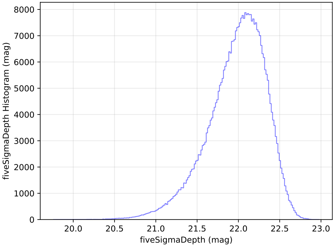
too_elab_r8_d3_giz_v3.4_10yrs All sky y band: fiveSigmaDepth Histogram
