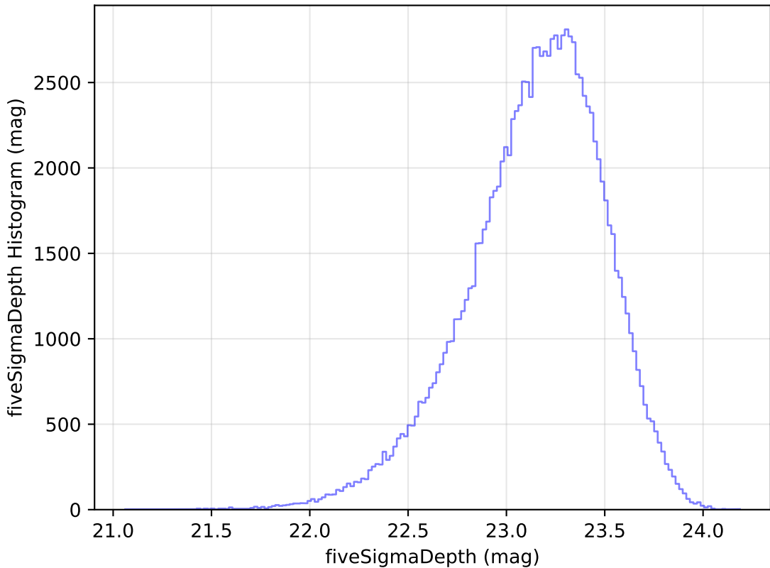
too_elab_r8_d3_giz_v3.4_10yrs All sky u band: fiveSigmaDepth Histogram
