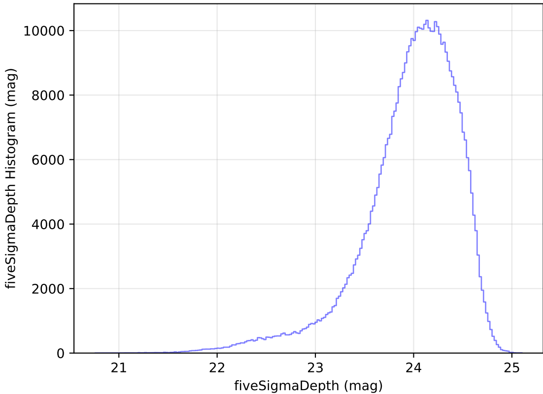
too_elab_r8_d3_giz_v3.4_10yrs All sky r band: fiveSigmaDepth Histogram
