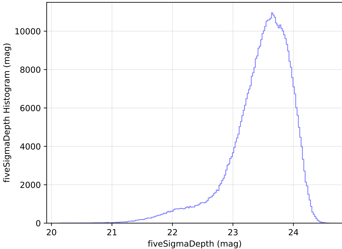
too_elab_r8_d3_giz_v3.4_10yrs All sky i band: fiveSigmaDepth Histogram
