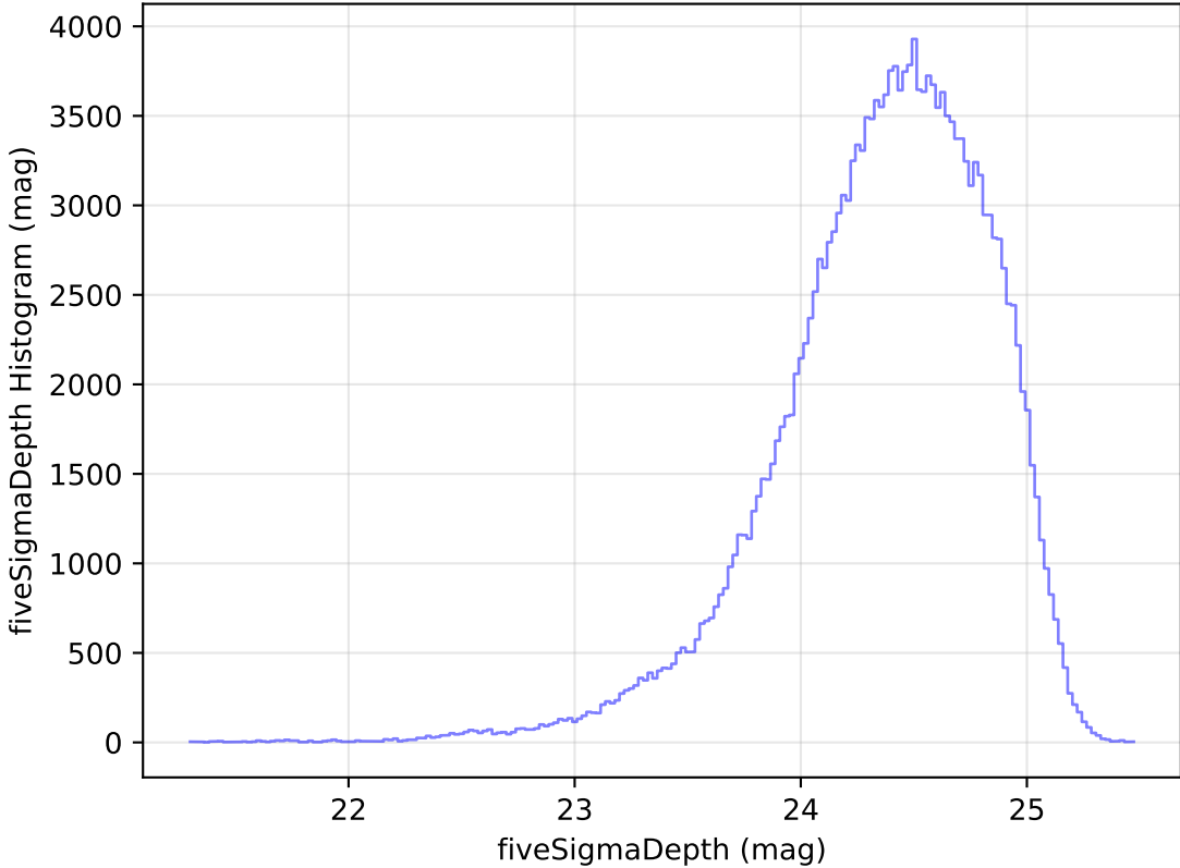
too_elab_r8_d3_giz_v3.4_10yrs All sky g band: fiveSigmaDepth Histogram
