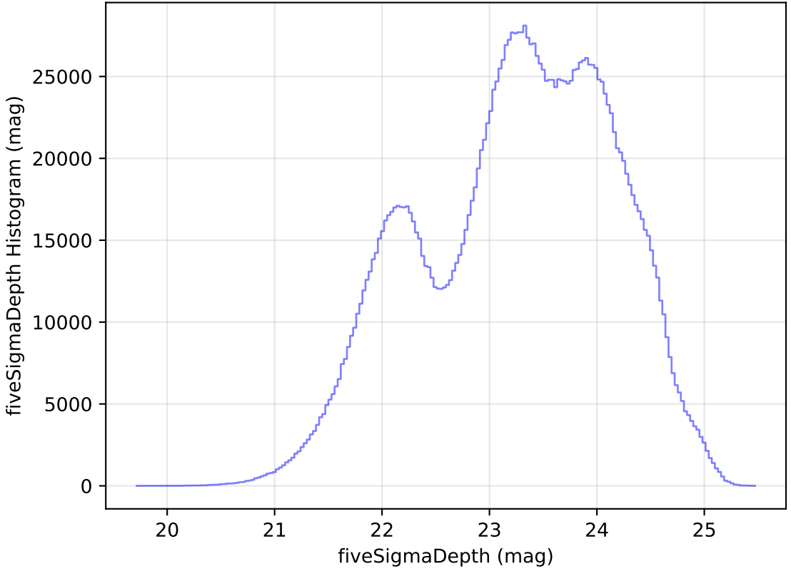
too_elab_r8_d3_giz_v3.4_10yrs All sky all bands: fiveSigmaDepth Histogram
