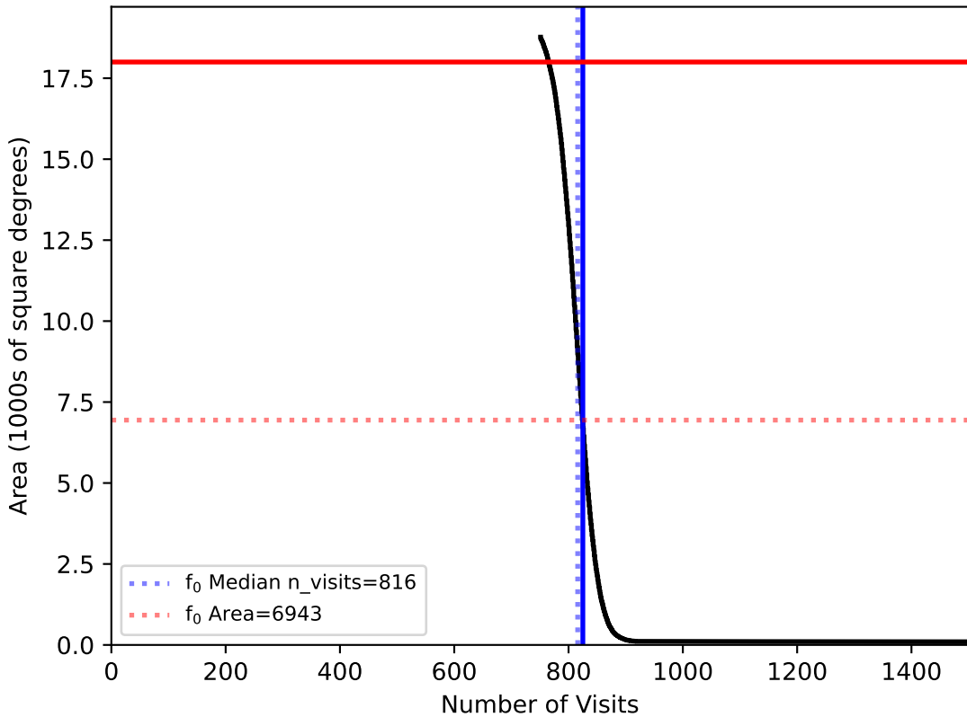
too_elab_r8_d3_giz_v3.4_10yrs WFD: fO
