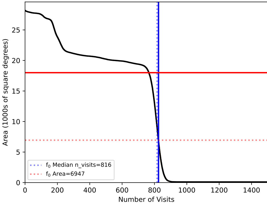
too_elab_r8_d3_giz_v3.4_10yrs All sky: f0
