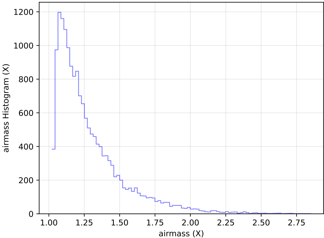
too_elab_r8_d3_giz_v3.4_10yrs Yr 1 u band: airmass Histogram
