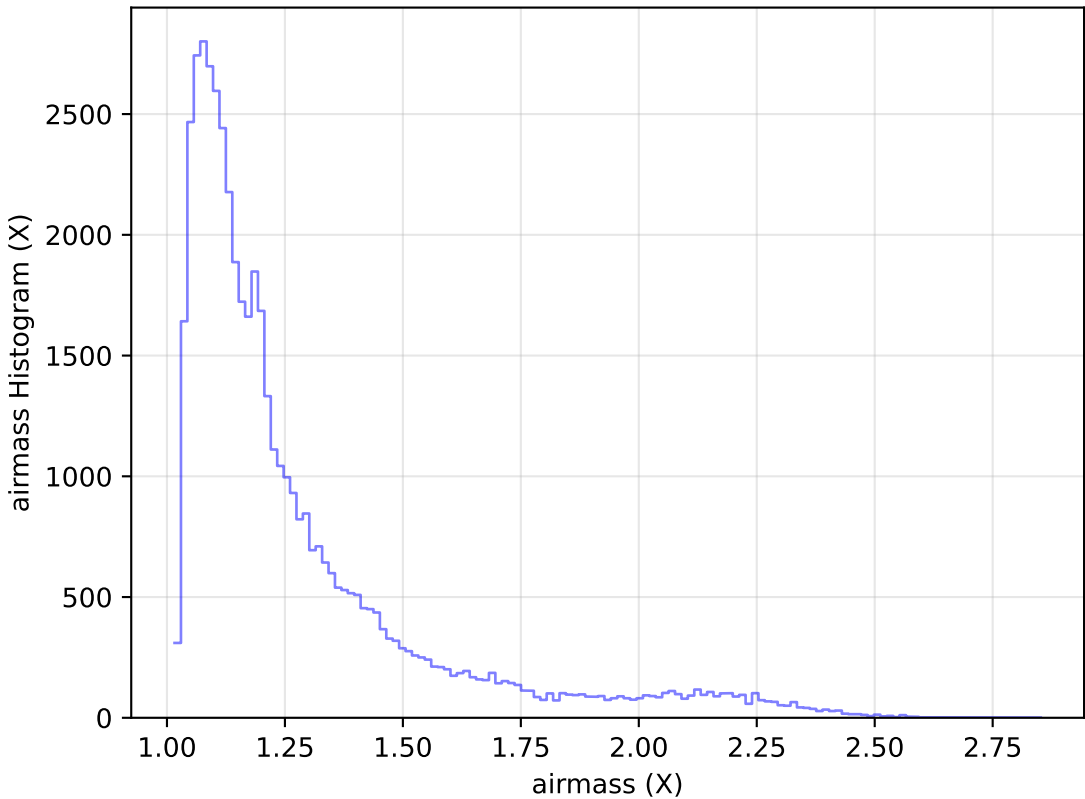
too_elab_r8_d3_giz_v3.4_10yrs Yr 1 r band: airmass Histogram
