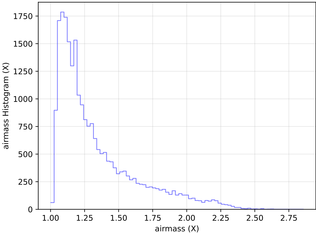
too_elab_r8_d3_giz_v3.4_10yrs Yr 1 g band: airmass Histogram
