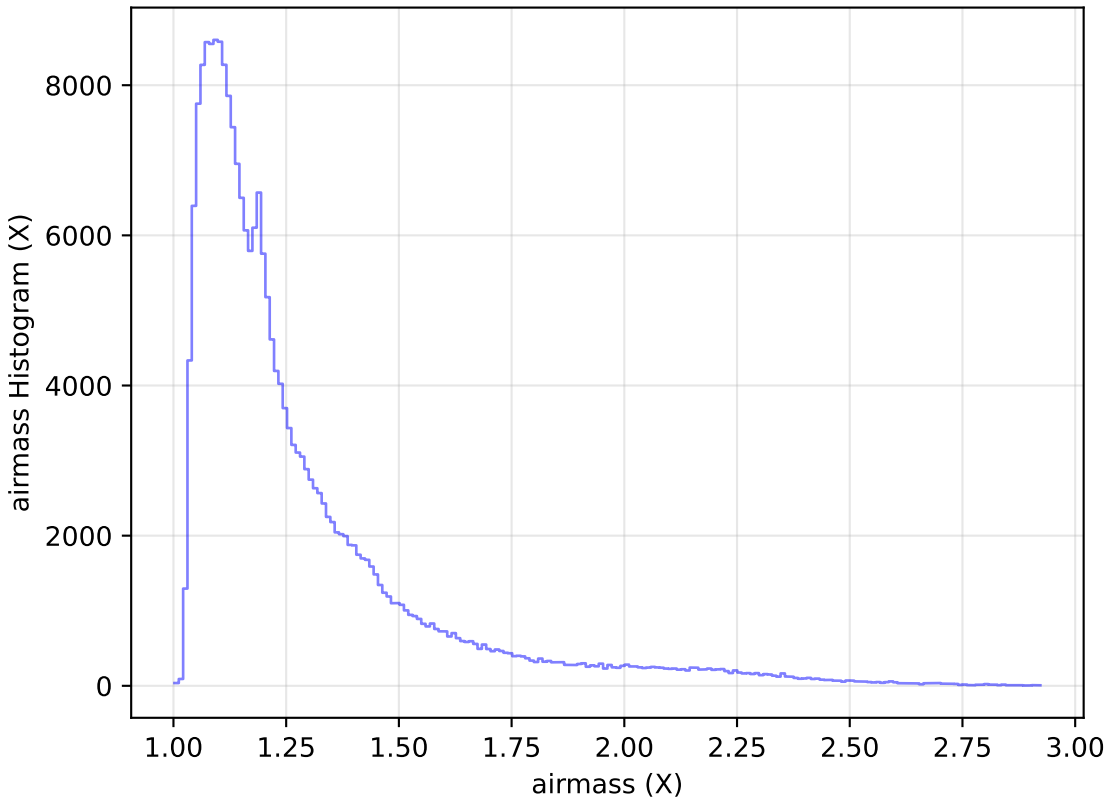
too_elab_r8_d3_giz_v3.4_10yrs Yr 1 all bands: airmass Histogram
