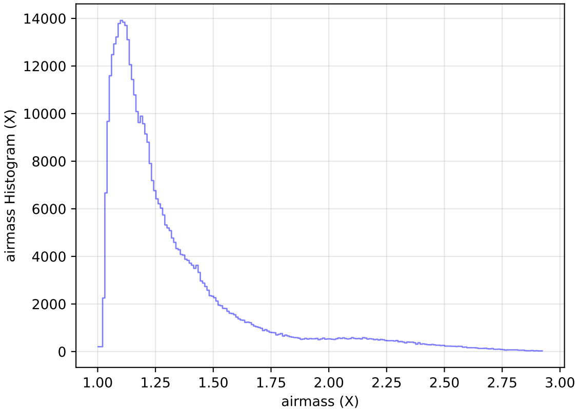
too_elab_r8_d3_giz_v3.4_10yrs WFD z band: airmass Histogram
