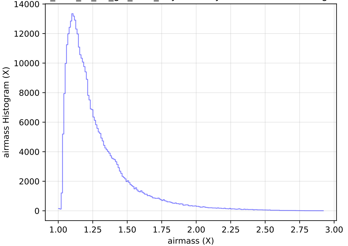
too_elab_r8_d3_giz_v3.4_10yrs WFD y band: airmass Histogram
