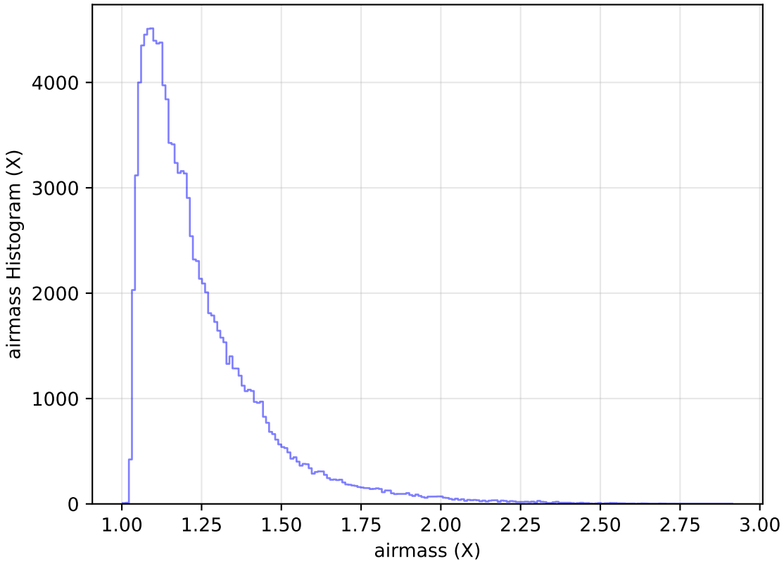
too_elab_r8_d3_giz_v3.4_10yrs WFD u band: airmass Histogram
