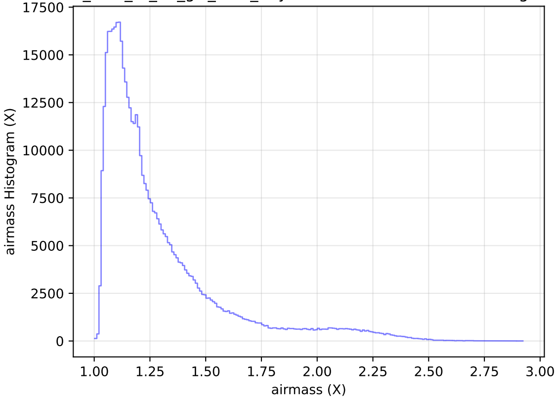
too_elab_r8_d3_giz_v3.4_10yrs WFD r band: airmass Histogram
