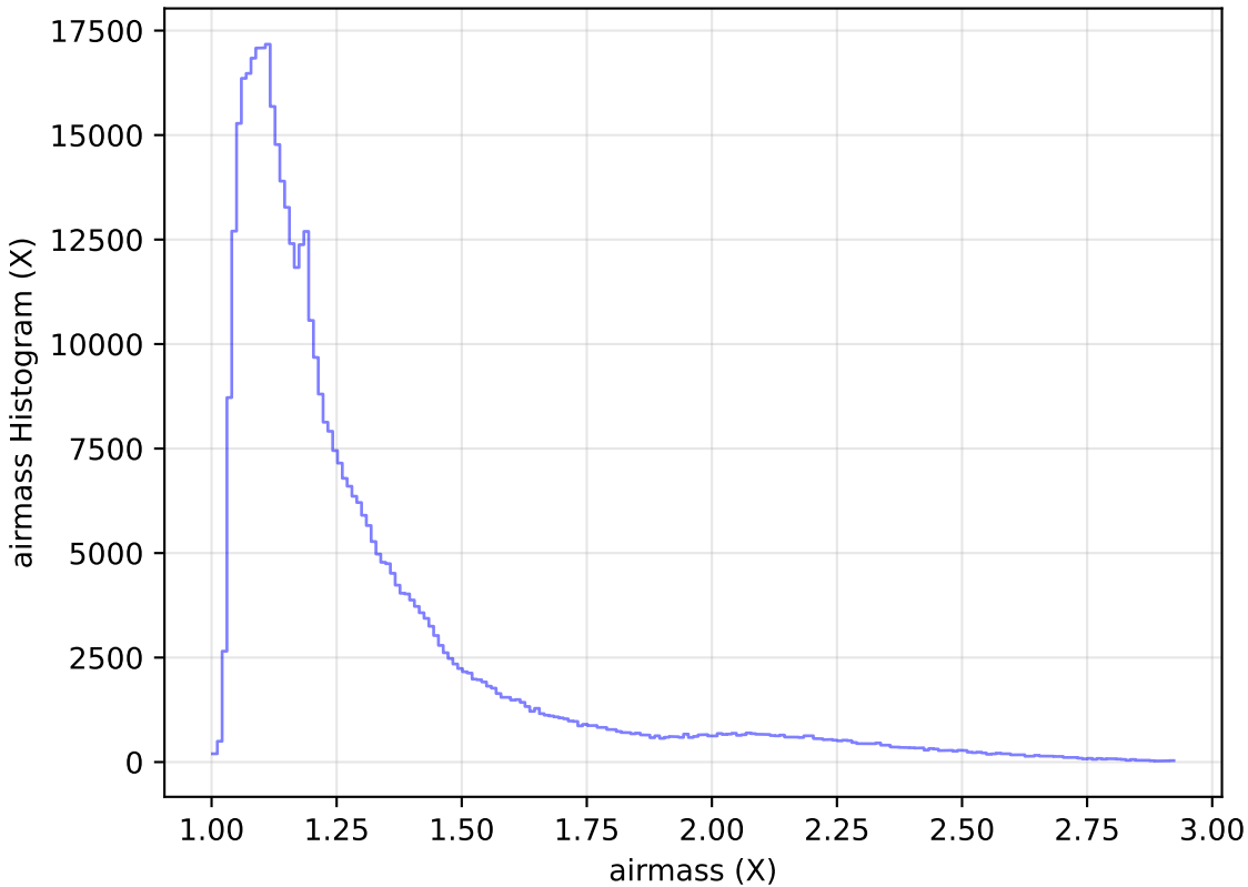
too_elab_r8_d3_giz_v3.4_10yrs WFD i band: airmass Histogram
