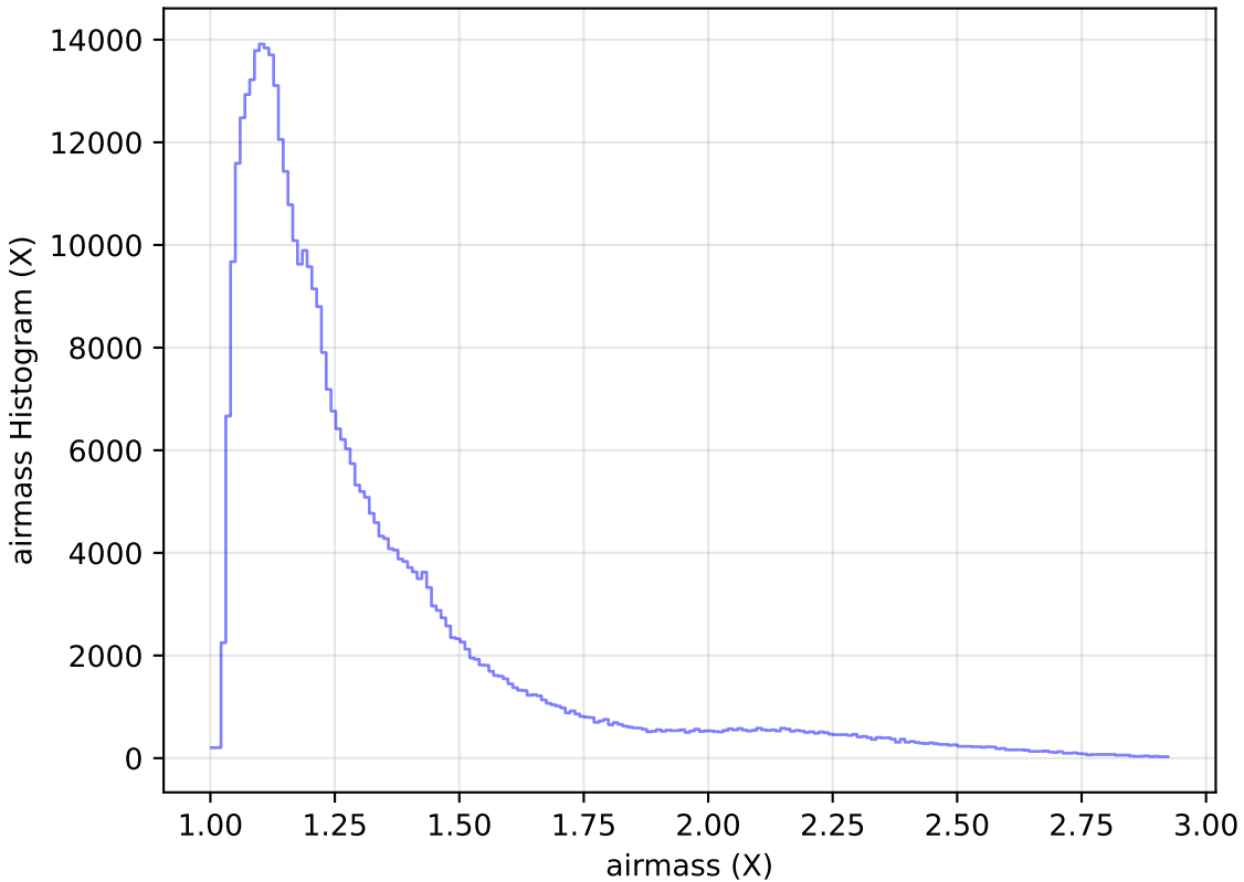
too_elab_r8_d3_giz_v3.4_10yrs All sky z band: airmass Histogram
