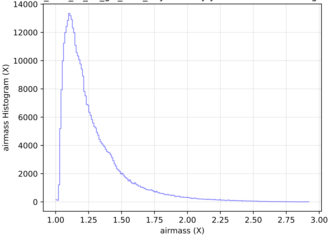
too_elab_r8_d3_giz_v3.4_10yrs All sky y band: airmass Histogram
