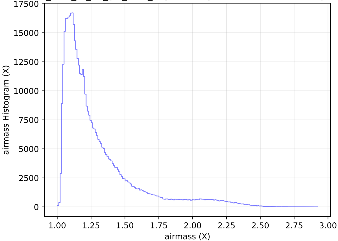
too_elab_r8_d3_giz_v3.4_10yrs All sky r band: airmass Histogram
