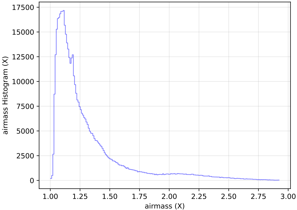
too_elab_r8_d3_giz_v3.4_10yrs All sky i band: airmass Histogram
