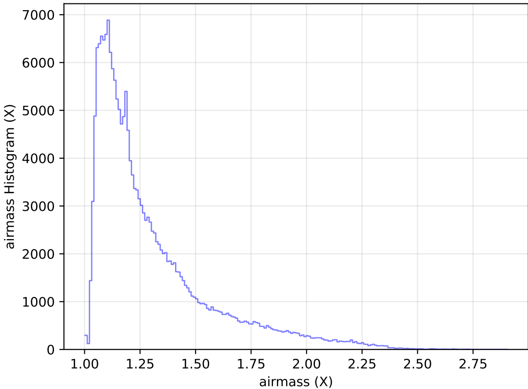
too_elab_r8_d3_giz_v3.4_10yrs All sky g band: airmass Histogram
