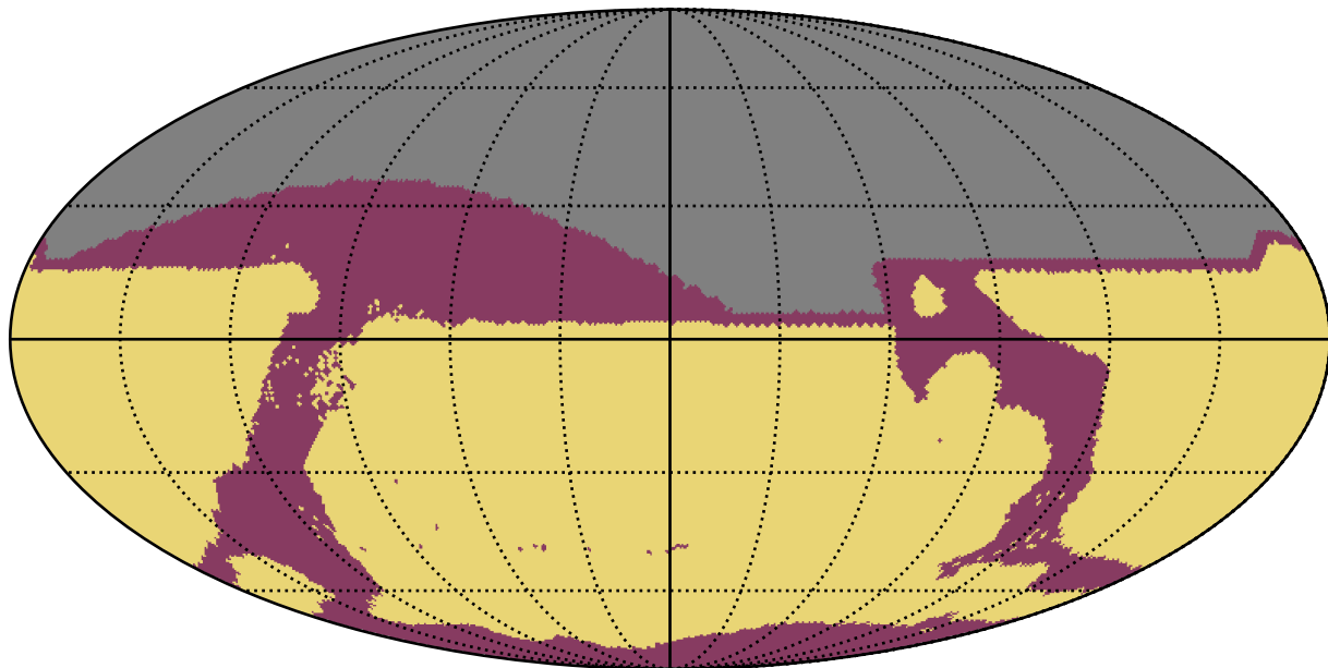
too_elab_r8_d3_giz_v3.4_10yrs All sky: RapidRevisits
