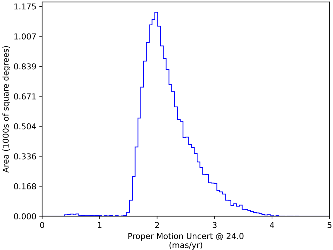
too_elab_r8_d3_giz_v3.4_10yrs WFD: Proper Motion Uncert @ 24.0
