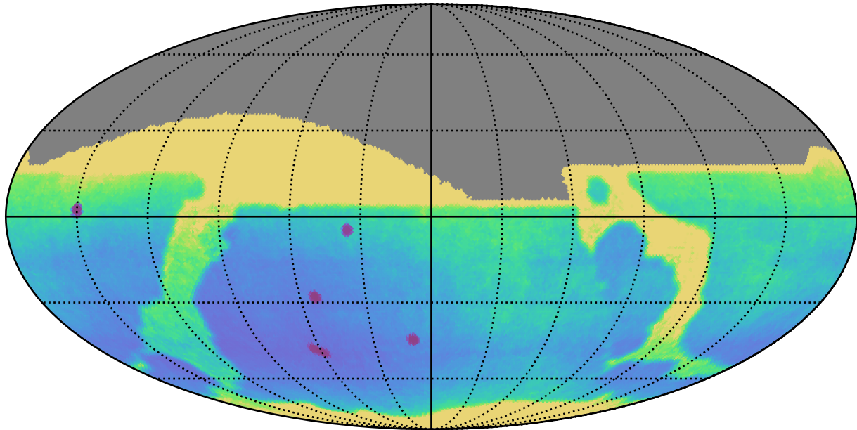
too_elab_r8_d3_giz_v3.4_10yrs All sky: Parallax Uncert @ 24.0
