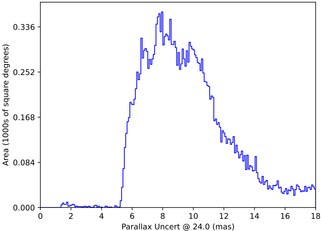
too_elab_r8_d3_giz_v3.4_10yrs All sky: Parallax Uncert @ 24.0
