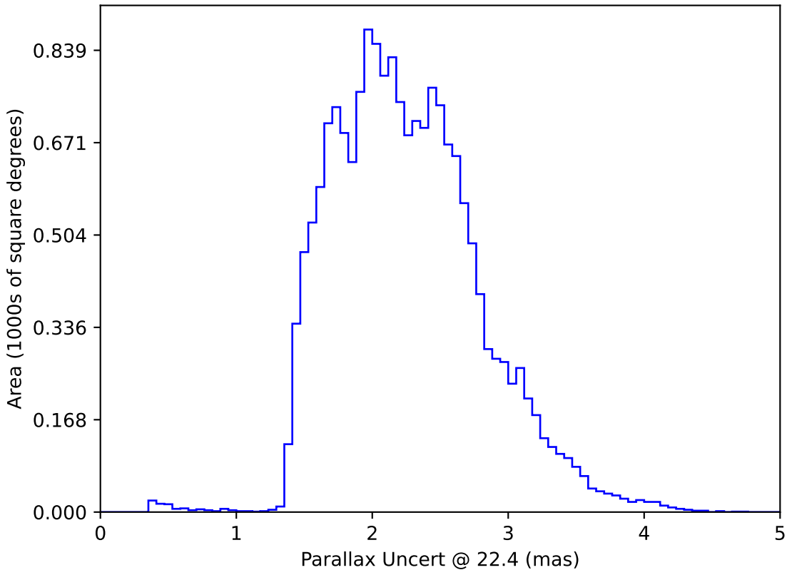
too_elab_r8_d3_giz_v3.4_10yrs WFD: Parallax Uncert @ 22.4
